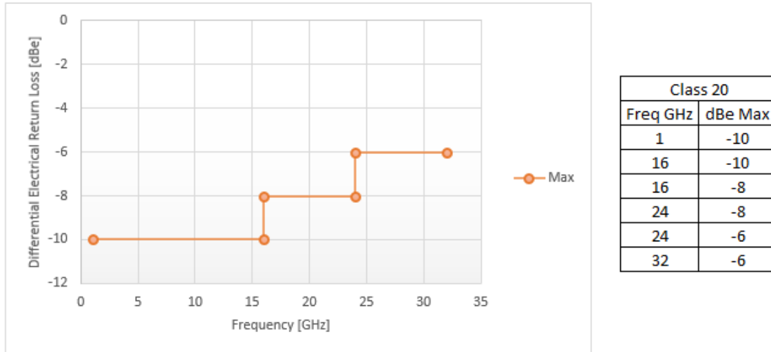
Figure 8-13: RX Class 20, Differential S22
